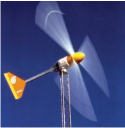
Capacity—10 kilowatts Turbine manufacturer—Bergey Windpower Company Photo credit—Bergey Windpower Company, NREL/PIX02102
